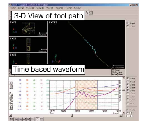
Tool path with time based waveform
