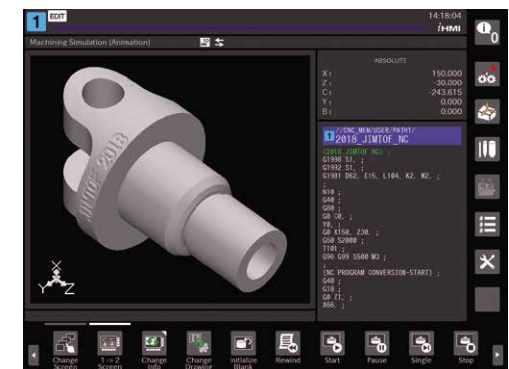
Machining program preview
